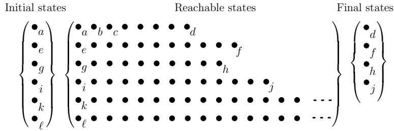
Fig. 5. Static / Collecting / Partial Correctness Semantics
